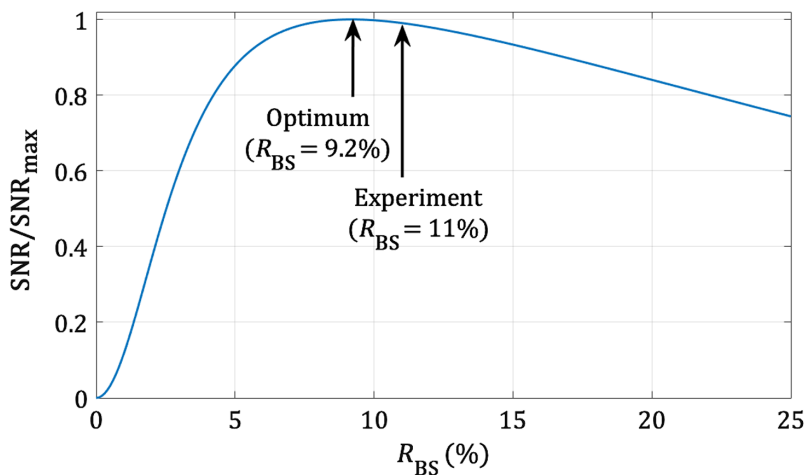
Fig. 4 Normalized theoretical SNR versus reflectivity of the beam-splitter ( R_{BS} ). Simulation based on Eq. (4), with the following parameters: R_{Ref} = 96\% and R_{S,inc} = 0.1\% . SNR is maximum for R_{BS} = 9.2\% . SNR/SNR_{max} = 0.99 for R_{BS} = 11\% (experiment).
