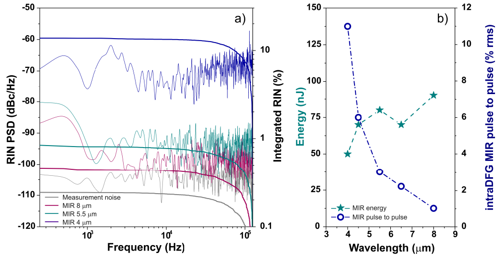
Fig. 7. (a) RIN measurements for the intraDFG source at 8 \mu\text{m} (red) 5.5 \mu\text{m} (green) and 4 \mu\text{m} (blue). (b) Pulse-to-pulse stability (blue) and pulse energy (green) as a function of MIR central wavelength.
