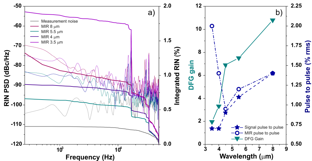
Fig. 8. (a) RIN measurements for the DFG source at 8 \mu\text{m} (red) 5.5 \mu\text{m} (green), 4 \mu\text{m} (blue), and 3.5 \mu\text{m} (violet). (b) Gain in the DFG crystal (green) and pulse-to-pulse stability of the seed at the input of the DFG (blue stars) and of the idler at the output of the DFG (blue circles).
