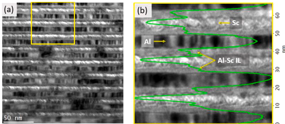
Fig. 3. Bright field TEM images of the 8028 Al/Sc sample prepared with mechanical flat-type tripod polishing. (a) is a 50k image and (b) is a 100k image of the selected area shown in (a), showing in detail the Al and Sc layers and Al-Sc interlayers (IL).
