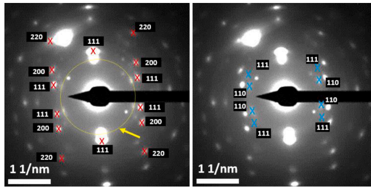
Fig. 4. 8028 Al/Sc multilayer electron diffraction images with identification of crystalline orientations for Al (left image) and Al 3 Sc (right image). Scandium layers are amorphous and appear as a diffuse circle as indicated on the left image.
