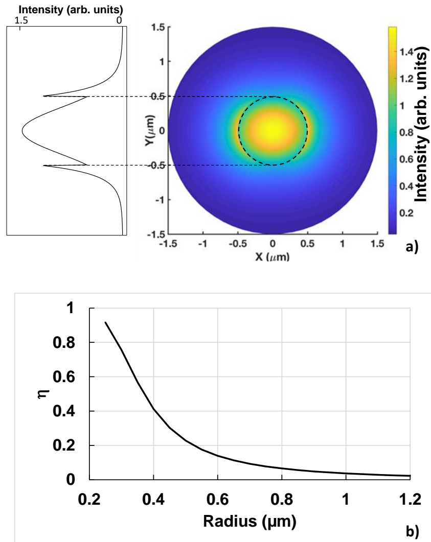
Figure 2. a) S_z , z-component of the Poynting vector of the fundamental mode HE11 at 1.5 μm for a nanofiber radius of 500 nm. The top panel is the S_z cross section in the plane Y=0 . The dashed line indicates the nanofiber diameter. b) Fraction of the evanescent field \eta versus the radius of the nanofiber at 1.5 μm.
