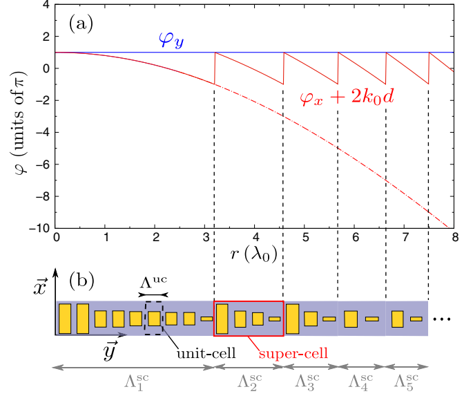
FIG. 4. Illustration of the phase-mapping approach for the 1D design of the resonant-phase delay metasurface. (a) Phase profiles to be encoded by the metasurface: the wrapped (respectively, unwrapped) spherical phase profile \phi_x of Eq. (17) (respectively, red full line) (respectively, red dashed line) desired for the x -polarization, and the flat phase profile \phi_y (blue line) desired for the y -polarization, starting from the center of the metasurface at r = 0 . (b) Corresponding nanoantennas to encode the desired phase shifts \phi_x and \phi_y . The unit cells of length \Lambda^{\text{uc}} (black dashed box) containing the nanoantennas are encompassed into supercells of length \Lambda^{\text{sc}} (red box), spanning the 2\pi phase space.
