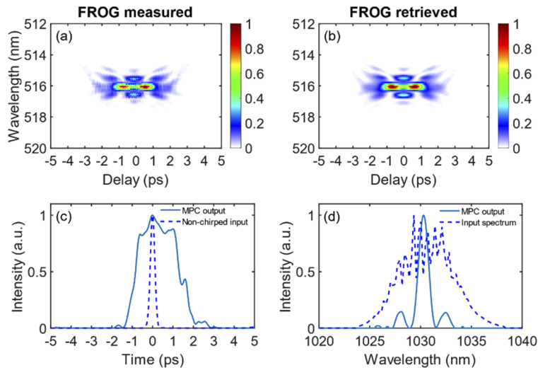
Fig. 3. (a) Measured and (b) retrieved FROG traces plotted in linear scale at the MPC output at 27 \mu\text{J} input energy; (c) FROG-retrieved temporal intensity profile (solid) at the MPC output and the temporal profile of the input laser pulse before negative chirping (dashed); (d) FROG -retrieved spectral intensity profile (solid) at the MPC output and spectrum of the input laser pulse (dashed).
