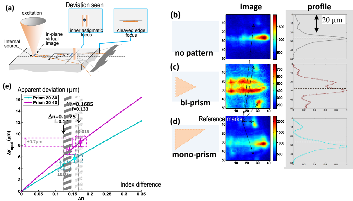
Figure 2: (a) Astigmatism in the beam seen on cleaved edge side; (b) images and averaged profile of virtual source seen without pattern, scale is in \mu\text{m} ; (c) same with a biprism 2x ( 10 \times 20 ) \mu\text{m} ; (d) same with a mono-prism 20 \times 30 \mu\text{m} ; (e) spot deviation vs. index difference of prism for two mono-prisms ( 20 \times 30 \mu\text{m} ) and ( 20 \times 40 \mu\text{m} ) and two hole sizes. Grey bands are the aggregate interval from both prism angles, for each hole size.
