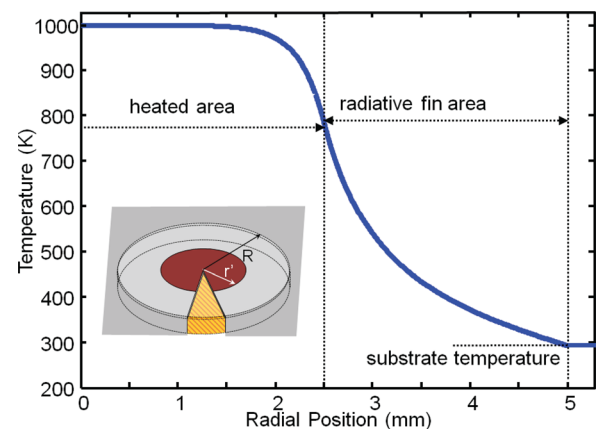
FIG. 4. Temperature distribution T(\mathbf{r}) for an encapsulated membrane ( R = 5 mm d = 350 nm) when the power is concentrated in a radius r' = 0.5R .
