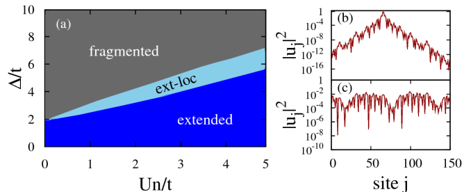
Figure 1. (Color online) Numerical results. (a) Localization diagram as a function of the interaction strength and the quasiperiodic amplitude. It displays three regimes: (i) 'extended regime' where the density background is connected and all excitations are extended; (ii) 'fragmented regime' where the density background is fragmented; and (iii) 'extended-localized regime' where the density background is connected and the excitation spectrum shows a delocalization-localization transition with exponentially localized high-energy states and extended low-energy states. (b)-(c) Typical excitation wave function u in the localized (b) and extended (c) regimes, plotted in semilogarithmic scale and for the 150 first lattice sites (similar plots are found for the v wave functions). The two panels correspond to two excitations with consecutive energies above (b) and below (c) the mobility edge for Un/t = 1.75t and \Delta/t = 3.3 .
