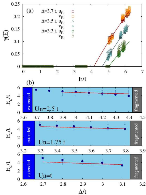
Figure 2. (Color online) (a) Lyapunov exponents of the Bogoliubov wave functions u and v , for U_n/t = 1.75 and \Delta/t = 3.3, 3.5, 3.7 . The excitation spectrum is banded and displays a sharp localization transition separating extended ( \gamma = 0 ) and localized ( \gamma > 0 ) states. (b) Mobility edge as a function of the quasiperiodic amplitude \Delta/t as extracted from power-law fits to the numerical \gamma(E) curves [solid lines on panel (a)]. Error-like bars correspond to the edges of the minigap containing the mobility edge. The dotted, red line shows the analytical prediction of the locator theory applied to the effective model (8) with the potential (11).
