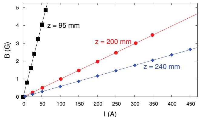
FIG. 6. Axial component of the magnetic field measured by the magnetoresistive magnetometer as a function of the current. Three different graphs are plotted, each corresponding to a different position z of the sensor with respect to the magnet. The best-fit straight lines to the points are also shown. For the last two positions, the AC power supply (50 Hz) was used, and the reported current and magnetic field values are rms.
