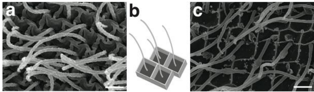
Figure 1. Scanning electron microscopy images of the Paramecium membrane for (a) a wild-type cell showing the pit structure of the membrane schemed in (b), and (c) a silenced cell showing the disruption of pits. Scale bar, 1 \mu\text{m} .
