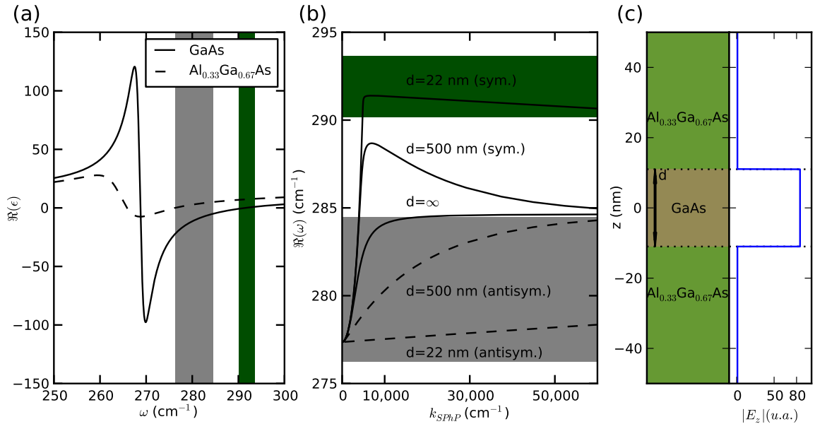
FIG. 1: (Color online) (a) Real part of GaAs and \text{Al}_{0.33}\text{Ga}_{0.67}\text{As} bulk dielectric functions as a function of the frequency. The gray area corresponds to the frequency range where an SPhP at the GaAs/ \text{Al}_{0.33}\text{Ga}_{0.67}\text{As} single interface can exist. The green (dark gray) shaded area correspond to the ENZ regime of GaAs, defined by K_{\text{ENZ}} = |\epsilon_{zz\text{AlGaAs}}/\epsilon_{zz\text{GaAs}}|^2 \geq 50 . (b) Dispersion relation for the slab geometry and different GaAs thicknesses d . The grey and green (dark gray) shaded areas have the same meaning as in Fig. 1a. When d=\infty , the system is similar to a single interface geometry. As the thickness is decreased, the mode separates into two branches (symmetric and antisymmetric normal electric field distribution [22, 23]). When d=22 nm, the symmetric branch frequency enters the ENZ regime of GaAs. (c) left: \text{Al}_{0.33}\text{Ga}_{0.67}\text{As}/\text{GaAs}/\text{Al}_{0.33}\text{Ga}_{0.67}\text{As} slab geometry, right: spatial distribution of the z -electric field component of the ENZ mode at 34.3 \mu\text{m} for a wavevector of 7000 \text{ cm}^{-1} and a GaAs thickness d of 22 nm.
