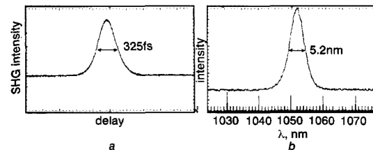
Fig. 2 Temporal and spectral characteristics of 210 fs pulses
