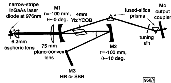
Fig. 1 Schematic diagram of low-threshold modelocked Yb:YCOB laser (not to scale)
