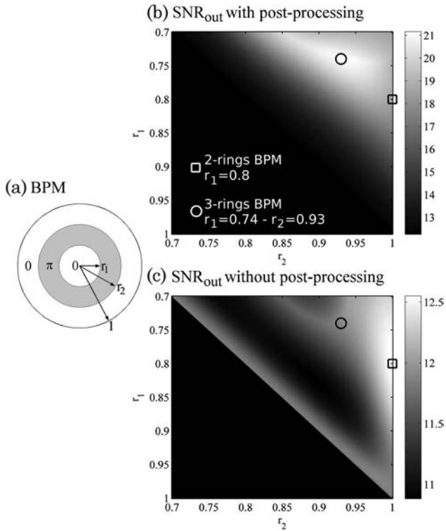
Fig. 1. (a) BPM structure and SNR out (dB) of the imaging system according to the BPM parameters (b) with and (c) without postprocessing and optimal BPM parameters.
