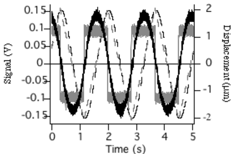
Figure 7 : Experimental response of the photorefractive velocimeter to a sinusoidal (black curves) and a sawtooth (grey curves) phase modulation of 0.6Hz frequency. The dashed lines represent the displacement of the piezomirror that creates the phase modulation.
