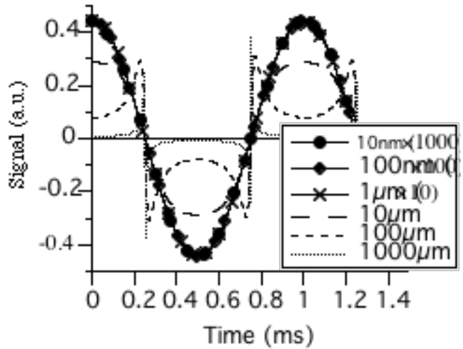
Figure 4 : Numerical simulation of the velocimeter response, for a sinusoidal displacement at 1kHz. The curves at the lowest amplitudes ( 0.01\mu\text{m} to 1\mu\text{m} ) are compensated for their amplitude. They superpose exactly showing the linearity of the response of the velocimeter.
