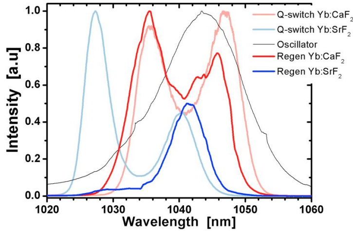
Fig. 13. Evolution of the spectrum in Q-switched and injected regime (blue and deep blue for Yb:SrF 2 , red and deep red for Yb:CaF 2 ), and oscillator spectrum (black)
