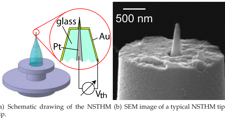
Fig. 8. Near field scanning thermal microscope developed in the group of Achim Kittel in Oldenburg (Kittel et al. (2008)). Reprinted with permission from Appl. Phys. Lett. , Vol. 93 , 193109 (2008). Copyright 2008, American Institute of Physics.
