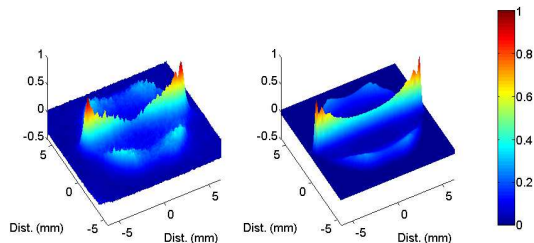
FIG. 23 Spatial profiles of the He* atom laser when the conditions for stimulated four wave mixing are met (experimental image - left, theoretical simulation - right). Four extra peaks, resulting from four wave mixing, are observed around the usual He* profile. Adapted from Dall et al. (2009).
