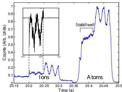
FIG. 18 Electron multiplier signal demonstrating stabilisation of the atom laser beam. The electron multiplier detects both the ions, which arrive first, and the beam of atoms, which arrives after a 150 ms time of flight. Feedback control is only implemented for the first half of the atom laser signal. The inset shows the closed-loop error signal (Dall et al. , 2008b). Reproduced with permission from The Optical Society (OSA).
