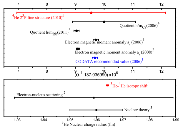
FIG. 15 Upper graph: Comparison of most updated \alpha determinations ( 1 Mohr et al. (2008) and references therein, 2 Hanneke et al. (2008), 3 Bouchendiria et al. (2011), 4 Gerginov et al. (2006)) with the recent \alpha value determined by 4 He 2^3\text{P}_0 - 2^3\text{P}_2 fine structure ( 5 Smiciklas and Shiner (2010)). Lower graph: Comparison of the {}^3\text{He} nuclear charge radius measured from the {}^3\text{He} - {}^4\text{He} isotope shift ( 1 Marin et al. (1995); Morton et al. (2006); Shiner et al. (1995); Zhao et al. (1991)) and by electron-nucleus scattering ( 2 Amroun et al. (1994)) and calculated by nuclear theory ( 3 Pieper and Wiringa (2001)).
