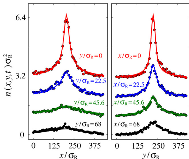
Figure 16. Experimental 2D column density distribution after 200 ms ( = 281\tau_R ) expansion of the atomic cloud. Dots are cuts along the x - (left panel) and y - (right panel) directions at cut positions explicitly indicated, artificially offset for clarity. Lines are the fitting function equation (36). Note that the spatial distribution is not Gaussian. This figure is reprinted from [77].
