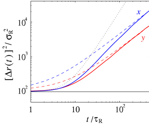
Figure 14. Mean square size, [\Delta r(t)]^2 , as a function of time, in the r = x (solid blue line) and r = y (solid red line) directions. The dotted line is equation (32) and has been obtained by assuming a ballistic expansion for all atoms. The dashed lines are equation (33), corresponding to all particles behaving diffusively. The horizontal line is the mean square size of the initial cloud, given by \sigma_T^2 . Here V_R = k_B T and \sigma_T = 10\sigma_R .
