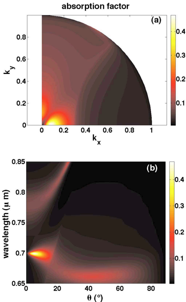
FIG. 3. (Color online) TM polarization. (a) Polar representation of the absorption factor for \lambda=700 nm of a silicon grating with period a = 0.54 \mu\text{m} , thickness t=0.1085 \mu\text{m} , and filling factor f=0.5 . (b) Absorption factor in the plane (\theta, \lambda) represented by linear color scale from bright (0.5) to dark (0).
