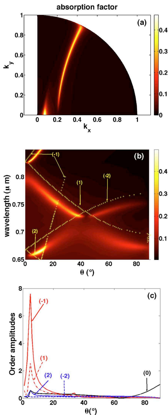
FIG. 2. (Color online) TM polarization. (a) Polar representation of the absorption factor for \lambda=830 nm of a silicon grating with period a = 0.54 \mu\text{m} , thickness t=0.1085 \mu\text{m} , and filling factor f=0.95 . (b) Dispersion relation of the unperturbed waveguide mode and absorption factor in the plane (\theta, \lambda) , respectively, represented by yellow markers +, and color scale from bright (0.5) to dark (0). (c) Amplitude of the -1, +1, -2, +2 diffracted orders (normalized to the amplitude of the incoming 0 order) vs the incident angle \theta for \phi=0^\circ , \lambda=830 nm. At this wavelength, only the 0 order is propagating.
