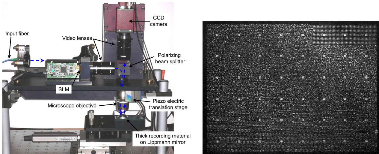
Fig 1.: Left : Lippmann data storage system, the blue dashed arrows represent the light path; Right: example of a retrieved data page with a 0.88\ \mu\text{m} pixel pitch.
